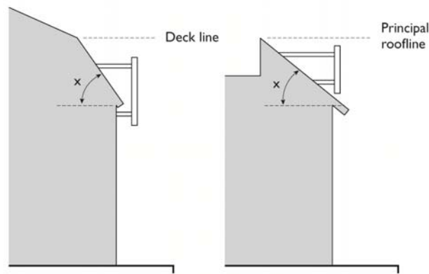
FIGURE 19.620.070.Q-5: MANSARD ROOF SIGN
